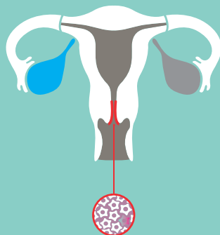
HPV VIRUS
